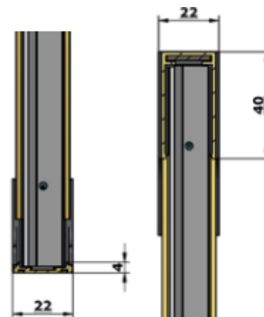
Section verticale
