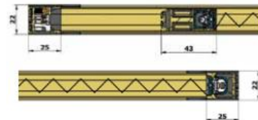
Section verticale
